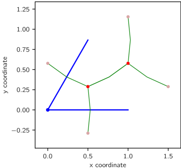
Graphene, bulk
