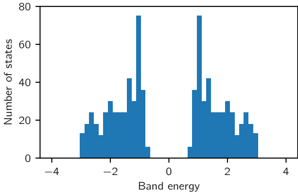
Finite Haldane model with PBC
