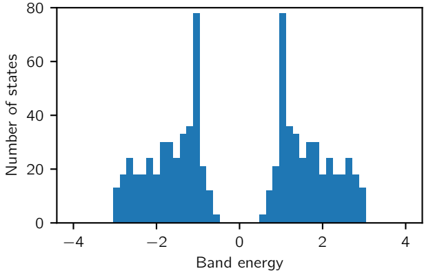
Haldane model density of states
