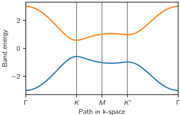
Haldane model band structure
