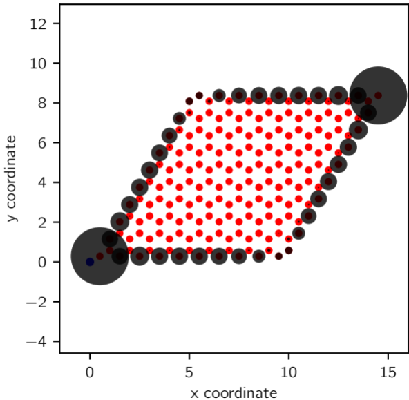
Edge state for finite model without periodic direction
