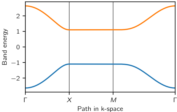
Checkerboard band structure
