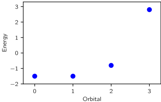
Molecule levels
