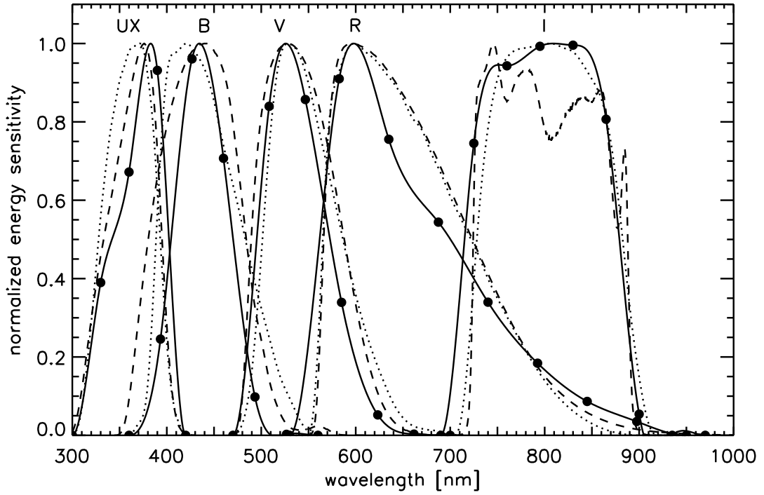
Fig. 4.— Model 4Shooter/Harris UBVRI passbands derived from observations of spectrophotometric standard stars ( solid curves ), calculated passbands from optics + filter transmission + detector response ( dashed curves ), and the standard UX and BVRI passbands of Bessell (1990; dotted curves ). The solid points show the location of the model spline points; see text for details.
