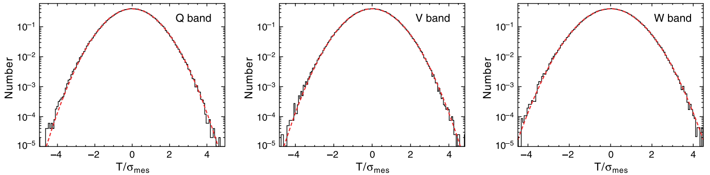
FIG. 22.—Normalized one-point distribution function of temperature anisotropy, defined in eq. (17), for the template-cleaned Q ( left ), V ( middle ), and W ( right ) band maps outside the Kp2 cut. The sky maps have been degraded to N_{\text{side}} = 256 for this figure. The red line shows the Gaussian distribution, which is an excellent fit to the one-point distribution function.
