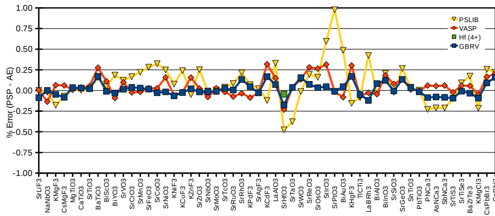
Figure 5: (Color online) Percent difference in AE versus pseudopotential calculations for perovskite (and anti-perovskite) lattice constants. GBRV potentials are blue squares, VASP potentials are red diamonds, PSLIB potentials are yellow triangles, and the \text{Hf}^{4+} potential is an isolated green square (see text).
