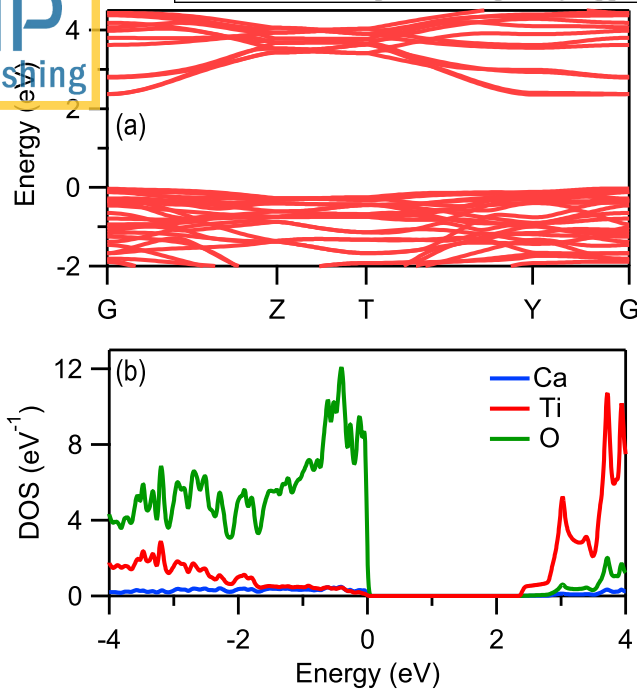
FIG. 3. (a) Band structure of \text{Ca}_3\text{Ti}_2\text{O}_7 . (See the Supplemental Information for the definition of the high symmetry points in the Brillouin Zone. 28,38 ) The bottom of the conduction band consists of dispersionless bands along the \Gamma -Y line (which is parallel to the crystallographic c axis), in line with the orbital projected DOS (shown in the supplemental material) that indicates that these bands consist of d -orbitals with lobes perpendicular to the c axis. (b) Densities of states per formula unit and projected onto the different atomic species.
