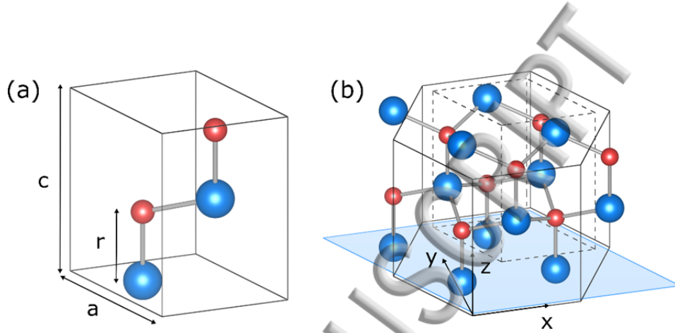
FIG. 2. (a) Wurtzite GaN unit cell and (b) crystal structure in which larger blue and smaller red spheres denote Ga and N atoms, respectively. Crystal structures were drawn with the VESTA visualization software [13].
