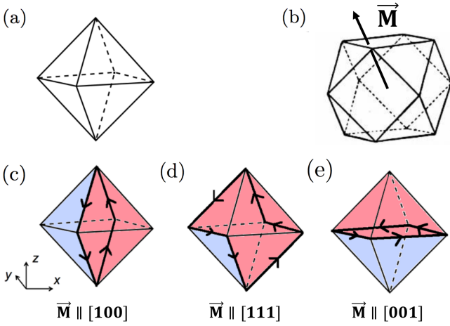
FIG. 10. Higher-order topological states at the surface of an FM axion insulator. (a) Octahedral crystallite with facets perpendicular to the [111] and equivalent directions. (b) Higher-order phase diagram. A given magnetization vector intersects the cuboctahedron at a particular face, with each face corresponding to a different arrangement of signs of the surface AHC on the crystallite. (c)-(e) Examples of surface configurations resulting from different magnetization directions. Color scheme follows that of Fig. 9.
