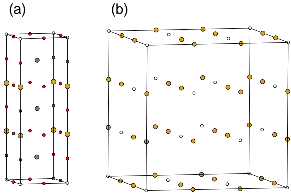
FIG. 1. (a) The 1:2_{[001]} \text{A}_3(\text{B}'\text{B}'')\text{O}_9 supercell. The succession of planes from bottom to top (i.e., progressing along [001] ) is (\text{B}',\text{O}) , (\text{Pb},\text{O}) , (\text{B}'',\text{O}) , (\text{Pb},\text{O}) , (\text{B}'',\text{O}) , (\text{Pb},\text{O}) ... (b) B-site atomic ordering in the 1:2_{[111]} structure, illustrated within a large box aligned with the cartesian axes. The succession of planes progressing along the [111] direction is (\text{B}') , (\text{Pb},\text{O}) , (\text{B}'') , (\text{Pb},\text{O}) , (\text{B}'') , (\text{Pb},\text{O}) ...; only \text{B}' and \text{B}'' atoms (small open and large filled circles respectively) are shown here.
