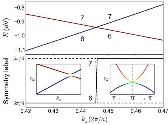
FIG. 7. (Color online.) A Weyl point between bands six and seven along the four-fold axis that projects onto \bar{M} in Fig. 3. The top panel and the right inset show the band dispersions as one passes through the touching point along the symmetry axis and on the orthogonal plane respectively. The left inset shows the dispersion along a vertical line that is shifted from the symmetry axis by \delta k_x = 0.05 \times 2\pi/a . The bands are color-coded by the spin as in Fig. 2. The main bottom panel shows the evolution along the symmetry axis of the phase of the C_4 eigenvalues (symmetry labels) of the crossing bands.
