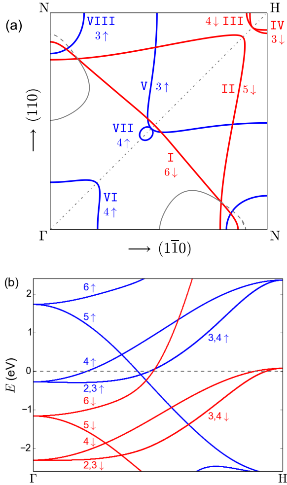
FIG. 9. (Color online.) (a) Fermi contours of bcc Fe on the \Gamma NH plane at k_z = 0 , calculated without spin-orbit coupling. The majority-spin contours I–IV are in red, the minority-spin contours V–VIII in blue. Curved grey lines are accidental degeneracy lines (nodal rings) that cross the Fermi level at points of contact between like-spin Fermi sheets, where they change from solid ( E_{\text{degen}} < E_F ) to dashed ( E_{\text{degen}} > E_F ). The dashed-dotted line from \Gamma to H is a line of essential degeneracy. (b) Energy bands close to the Fermi level along the \Gamma H line. In both panels, the spin-dependent band indices are indicated.
