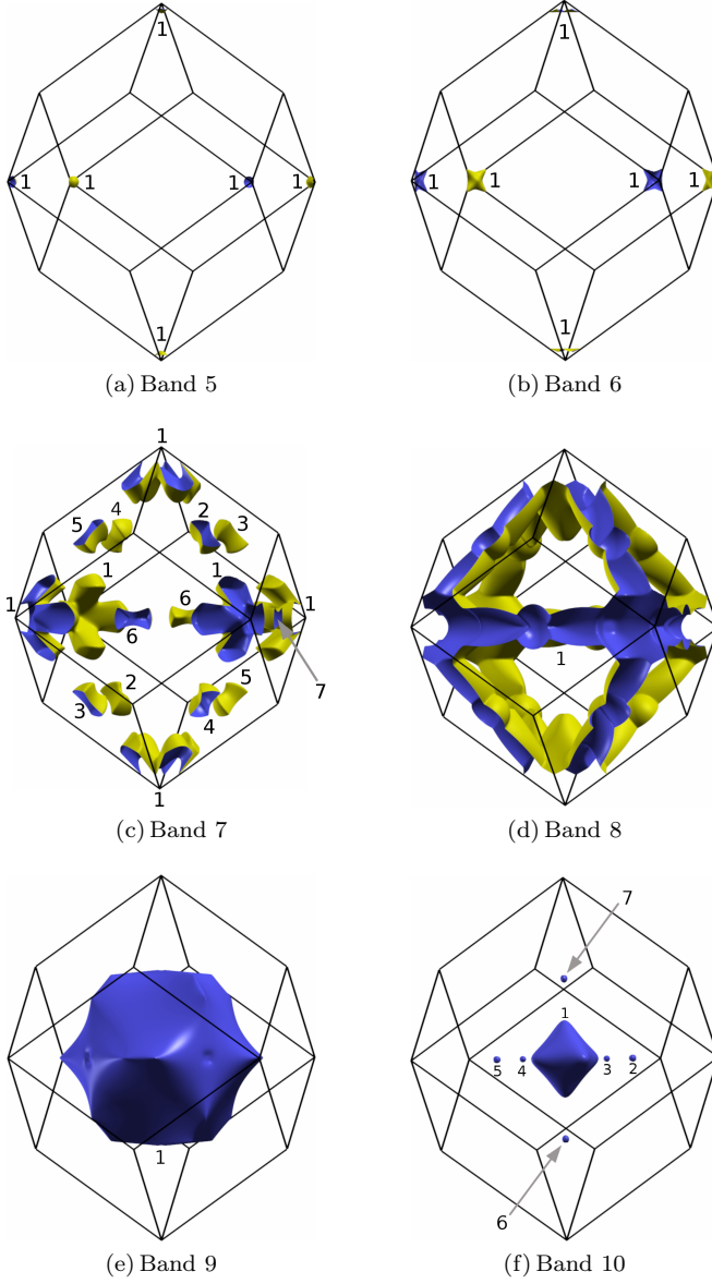
FIG. 10. (Color online.) Fermi surface of bcc Fe with spin-orbit coupling included. The indices a of the individual Fermi sheets S_{na} on each band n are indicated.
