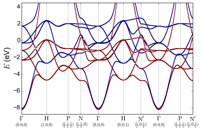
FIG. 2. Bandstructure of bcc Fe with spin-orbit coupling included. Energies are measured from the Fermi level, and the bands are color-coded by the expectation value of the spin component S_z , ranging from red (majority down-spin character) to blue (minority up-spin).
