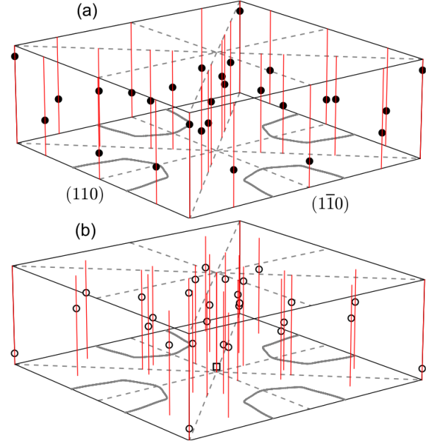
FIG. 4. (Color online.) Degeneracies between bands six and seven in the half Brillouin zone of Fig. 3. (a) Black dots denote Weyl points of positive chirality (monopole sources of Berry curvature on band six). (b) Open circles denote Weyl points of negative chirality, and the single open square represents a negative double-Weyl node. Each chiral degeneracy is threaded by a vertical line to help locate it with respect to the projected high-symmetry lines (dashed grey lines). The solid grey lines on the k_z = 0 plane represent nonchiral nodal rings.
