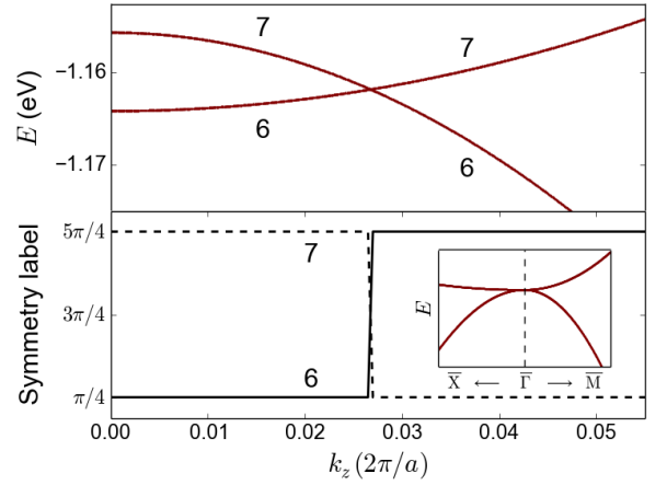
FIG. 8. (Color online.) A double-Weyl node between bands six and seven along the four-fold axis \Delta in Fig. 3. The top and bottom panels and the right inset have the same meaning as in Fig. 7. Near the crossing the two bands have majority-spin character, as indicated by the red color.
