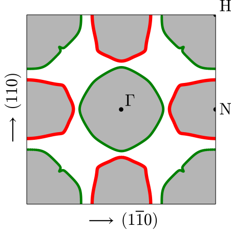
FIG. 5. (Color online.) Mirror symmetry labels (+ i in grey and -i in white) of band six on the mirror plane at k_z = 0 . The degeneracy lines of band six with bands five and seven are drawn in thin (green) and thick (red) lines respectively.
