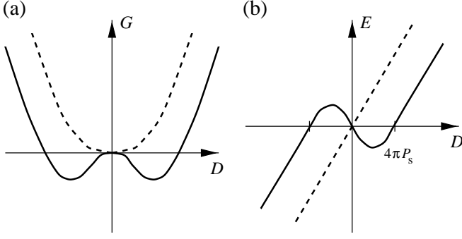
FIG. 2. Sketch of the Gibbs free energy G and the internal electric field E as a function of the dielectric displacement D (or the external electric field E_{\text{ext}} , respectively) for a paraelectric (dotted line) or ferroelectric (solid line) slab.
