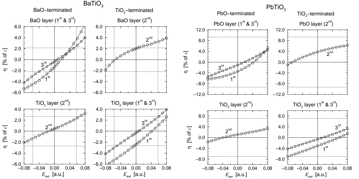
FIG. 7. Field dependence of the rumpling parameter \eta_i calculated from the 7-layer slab. Dotted horizontal lines: amplitude of displacement of metal and oxygen ions in the bulk ferroelectric state. Dotted vertical lines: External electric field corresponding to the bulk spontaneous polarization.
