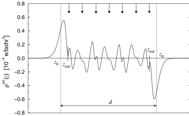
FIG. 5. Planar-averaged screening charge distribution of a BaO-terminated slab of BaTiO 3 , calculated from a 7-layer slab for an electric field of E_{\text{ext}} = +0.02 a.u. The arrows indicate the positions of the atomic planes. “Top” of slab is at right.
