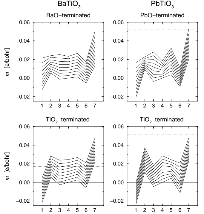
FIG. 9. Dipole moment per atomic layer calculated for the 7-layer slabs for electric fields from 0 to 0.08 a.u. in steps of 0.01 a.u. The orientation of the electric field corresponds to a positive field for the top surface and a negative field for the bottom surface. The dotted line represents the dipole moment for an atomic layer in the bulk ferroelectric state, calculated from the bulk spontaneous polarization via c/2 \cdot P_s^{\text{bulk}} .
