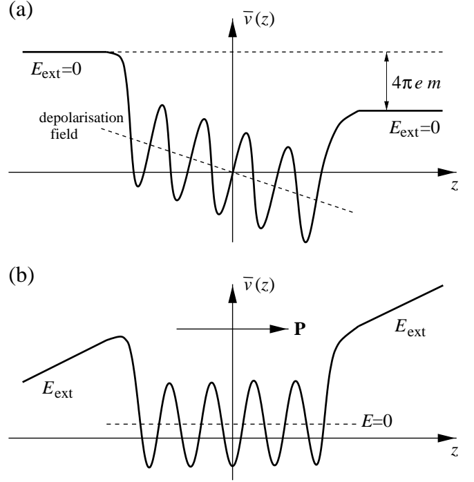
FIG. 1. Schematic illustration of the planar-averaged potential \bar{v}(z) for an isolated slab with a dipole moment m perpendicular to the surface. (a) Vanishing external electric field (equivalent to D=0 ). (b) Vanishing internal electric field ( E=0 ).
