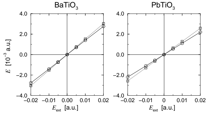
FIG. 6. Internal electric field E in the 7-layer slab with frozen atomic positions as a function of the applied external electric field E_{\text{ext}} . Solid lines: AO-terminated slabs. Dotted lines: TiO 2 -terminated slabs. Atomic units are used. 18
