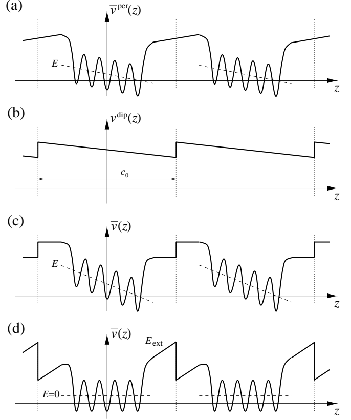
FIG. 3. Schematic picture of the planar averaged potential \bar{v}(z) for periodically repeated slabs. (a) with periodic boundary conditions, (b) potential of the dipole layer, (c) dipole corrected slabs with vanishing external electric field, (d) dipole corrected slabs with vanishing internal electric field.
