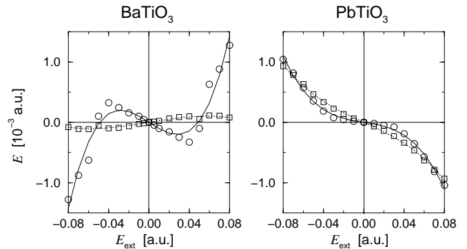
FIG. 10. Internal electric field E in the fully relaxed 7-layer slab as a function of the applied external electric field E_{\text{ext}} . Solid lines, AO-terminated slabs; dotted lines, TiO 2 -terminated slabs.
