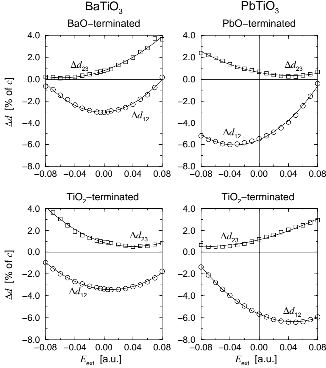
FIG. 8. Field-dependence of the change in interlayer distances \Delta d_{ij} calculated for the 7-layer slabs.
