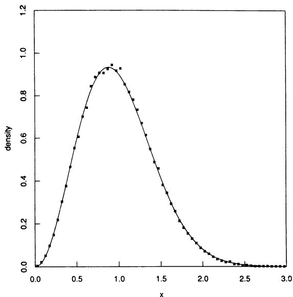
Nearest neighbor spacings, N = 10^{12}
