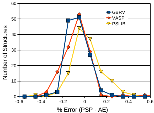
FIG. 6: (Color online) Histogram of % error in lattice constants (PSP - AE) for the half-Heusler test set. GBRV results in blue squares, VASP in red diamonds, and PSLIB in yellow triangles.
