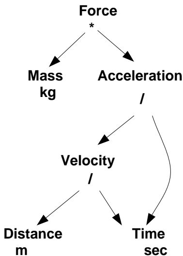
Figure 2: Physics Concepts and Their Relationship To One Another
