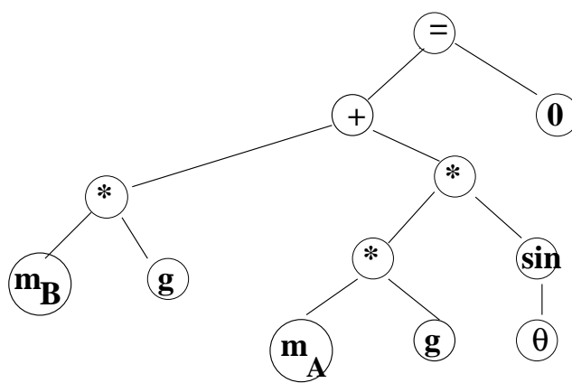
Figure 6: Parse Tree Of An Incorrect Answer
