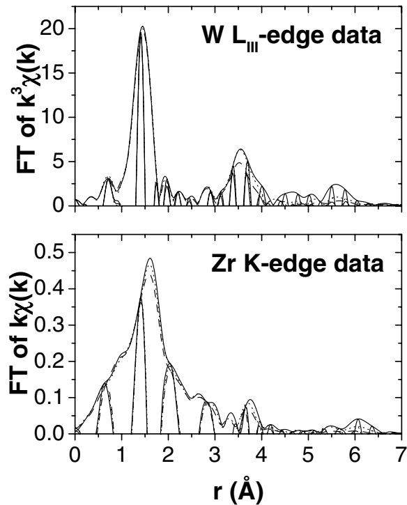
FIG. 1. XAFS r -space data for both W L_{III} - and Zr K -edge data up to 7 Å. Data at 20 K (solid line), 160 K (dotted line), and 315 K (dashed line) are shown for each edge. The Fourier transform (FT) range is from 3.3 to 13.5 Å -1 , with 0.3 Å -1 Gaussian broadening. The high frequency curve inside the envelope is the real part of the Fourier transform ( FT_R ). The envelope is defined as \pm\sqrt{FT_R^2 + FT_I^2} , where FT_I is the imaginary part of the transform. There is a well-defined XAFS phase shift for each peak, consequently the nearest W-O peak occurs at \sim 1.4 Å (upper panel), the nearest W-Zr peak (including W-O-Zr multiple-scattering contribution) shifts to about 3.5 Å, and the nearest W-W peak is around 3.9 Å. In the bottom panel, the nearest Zr-O peak is at 1.6 Å; the nearest Zr-W peak (including Zr-O-W linkage) shifts to about 3.75 Å; the nearest Zr-Zr peak is near 6.0 Å.
