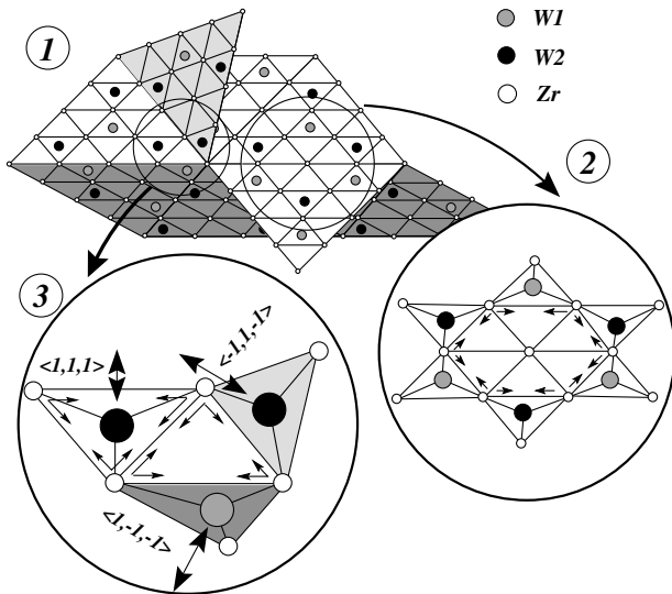
FIG. 4. A sketch of part of the crystal structure with only W and Zr atoms plotted (O atoms are omitted for clarity). The white, light gray, and dark gray planes are three different planes perpendicular to \langle 1, 1, 1 \rangle , \langle -1, 1, -1 \rangle , and \langle 1, -1, -1 \rangle axes, respectively. Zr atoms are at the corner of each triangle, while W atoms are at the center of every thick-line triangle (filled triangle). Panels 2 and 3 show the detailed structure of small parts of panel 1, in which the W-O-Zr linkage is shown by a thin black solid line. Panel 2 shows part of the white plane with six connected filled triangles surrounding a hexagon formed by six nonfilled triangles. The thick arrows in panel 3 show the vibration direction of each W atom.
