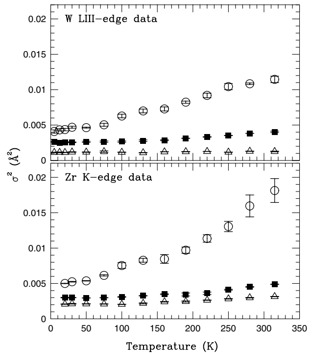
FIG. 2. \sigma^2 vs temperature. The W L_{III} -edge data are plotted in the upper panel: the open triangles represent the nearest neighbor W-O bonds; the solid squares show \sigma^2 for the W-Zr pair including W-O-Zr multiple-scattering effects; the open circles represent the nearest W(1)-W(2) atom pair. In the lower panel, \sigma^2 for three atom pairs are shown: the nearest neighbor Zr-O bond (open triangle), the nearest Zr-W pair including the Zr-O-W linkage (solid square), and the nearest Zr-Zr pair (open circle). Note the unusual cusp for the W-W and Zr-Zr pair data near 100 K.
