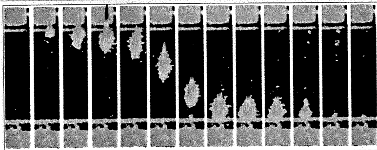
Ambipolar carbon-nanotube transistors can emit light when electrons (travelling from the top in this figure) recombine with holes (from below). The advantage of this type of device over, say, light-emitting diodes is that the origin of the light can be moved simply by changing the gate voltage. Carbon nanotubes could therefore be used as ultrasmall adjustable light sources.
