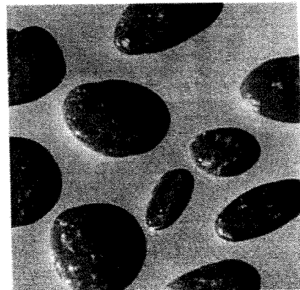
fractured iridescent green butterfly scale (center) shows the submicron-size face-centered cubic structure inside. Opals consist of submicron-size silica spheres arranged in a face-centered cubic [close-packed] structure.
