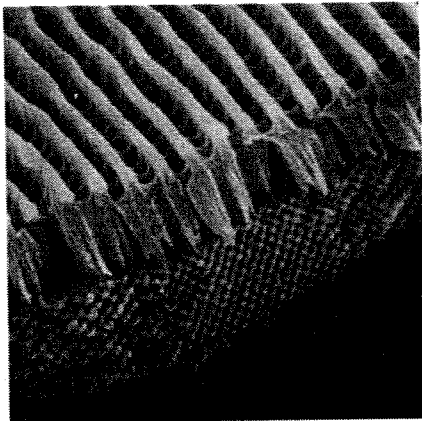
fractured iridescent green butterfly scale (center) shows the submicron-size face-centered cubic structure inside. Opals consist of submicron-size silica spheres arranged in a face-centered cubic [close-packed] structure.
