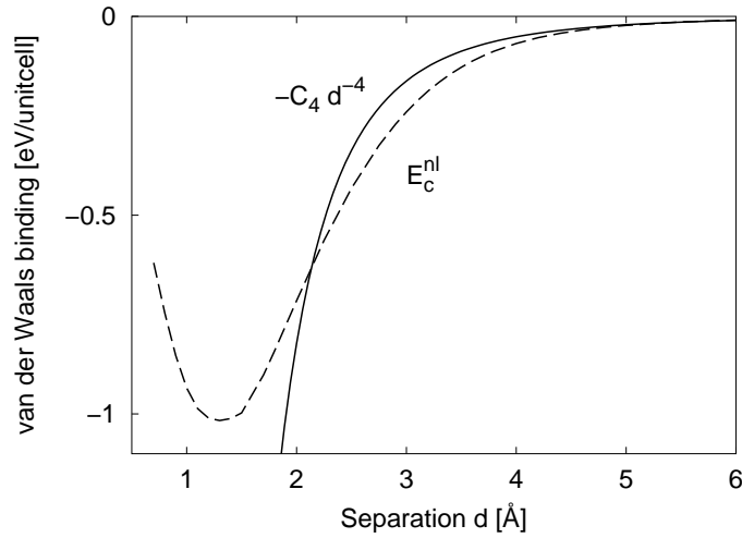
Figure 3: Enhancement and eventual saturation of the nonlocal-correlation energy contribution E_c^{\text{nl}} evaluated for a pair of graphene sheets as a function of the interlayer separation d . One unit cell contains two sheets, each with two carbon atoms.
