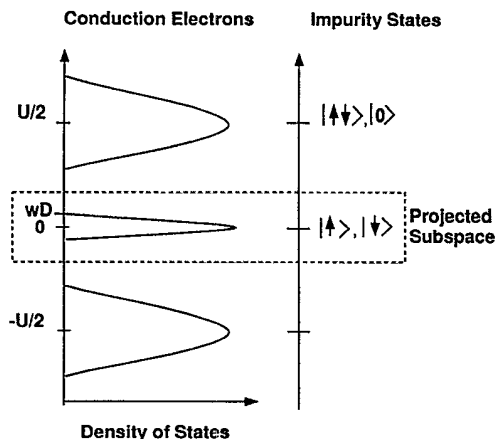
FIG. 1. Schematic plot of the spectral functions of the conduction electrons and the impurity configurations, illustrating the narrow low-energy and broad high-energy parts.
