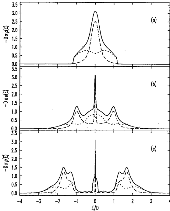
FIG. 4. (a) Single-particle density of states (DOS) as a function of energy (after analytical continuation i\omega_n \rightarrow E + i\eta ), in the weak correlation regime U/D = 0.1 . The average DOS is shown by a full line, whereas the partial DOS's corresponding to the A and B sites (see text) are plotted by dashed and dotted lines, respectively. (b) Intermediate correlation U/D = 1.6 . Note that the partial DOS of the A site (dashed line) has a form characteristic of a local moment, with the upper and lower Hubbard bands appearing, and a sharp Kondo resonance at the Fermi surface. The B sites (dotted line) are still itinerant. (c) DOS close to the Mott transition, U/D = 3.2 (strong correlations). In this regime, all sites are in the local moment regime, but with different Kondo temperatures T_K^A \ll T_K^B . The system is still metallic due to the Kondo delocalization.
