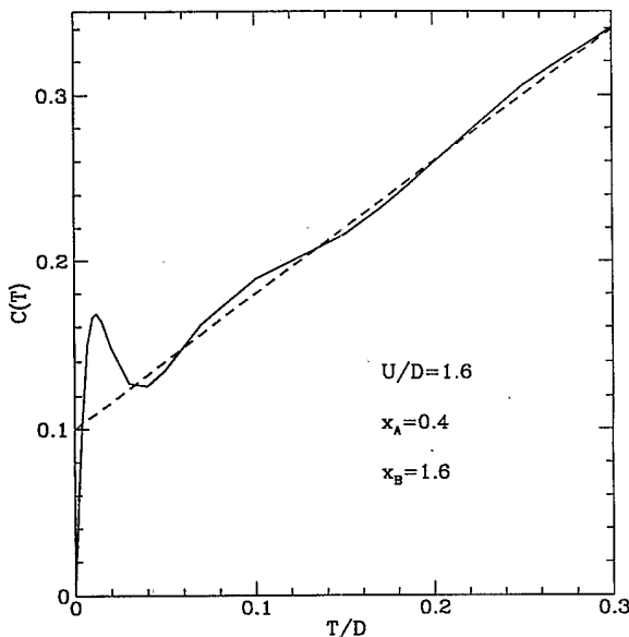
FIG. 6. The specific heat for the binary model of hopping randomness, at an intermediate correlation corresponding to coexistence of local moments and conduction electrons [as in Fig. 4(b)]. Fermi-liquid behavior (linear specific heat) occurs at low temperatures T < T_k^A \sim 0.01D . At higher temperatures, the temperature dependence is reminiscent of the phenomenological two-fluid model (Ref. 14) of doped semiconductors [see Eq. (64)].
