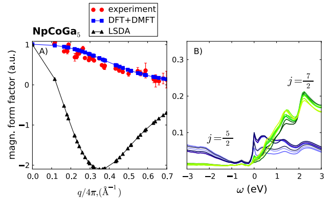
FIG. 1 (color online). (a) Magnetic form factor for NpCoGa 5 . Red dots are experimental data reproduced from [6]. The blue curve with squares is the DFT + DMFT calculation, and the black curve with triangles is the LSDA calculation. The DFT + DMFT form factor agrees with experiment with the value of the Pearson correlation coefficient R_{\text{PMCC}} = 0.95 . (b) Spectral function A_{jm_j}(\omega) for Np f electrons. Blue (dark gray) curves correspond to the j = 5/2 multiplet and green (light gray) curves to the j = 7/2 multiplet. The experimental and theoretical DMFT temperature is T = 52 K.
