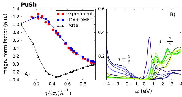
FIG. 2 (color online). (a) Magnetic form factor for PuSb at T = 20 K. Red dots are experimental data [27], the blue curve with squares is the DFT + DMFT calculation and the black curve with triangles the LSDA calculation. The DFT + DMFT curve agrees with experiment with a Pearson correlation coefficient R_{\text{PMCC}} = 0.95 . (b) Spectral function for PuSb. The color legend is the same as in Fig. 1.
