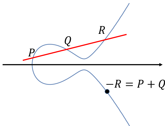
Figure 3: In a suitable range of real values of f, g the real points on the elliptic curve have the above form. Then the elliptic curve group law is easily pictured as shown.
