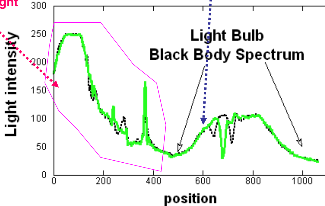
Diffraction grating spectrum of incandescent light bulb – black body spectrum. of
