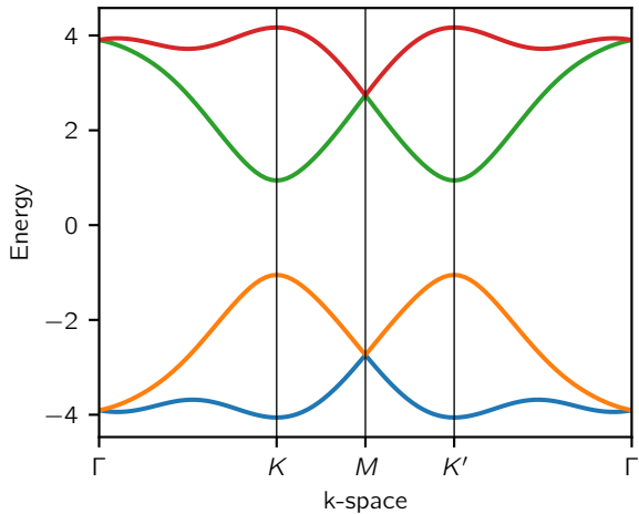
Kane-Mele: even phase
