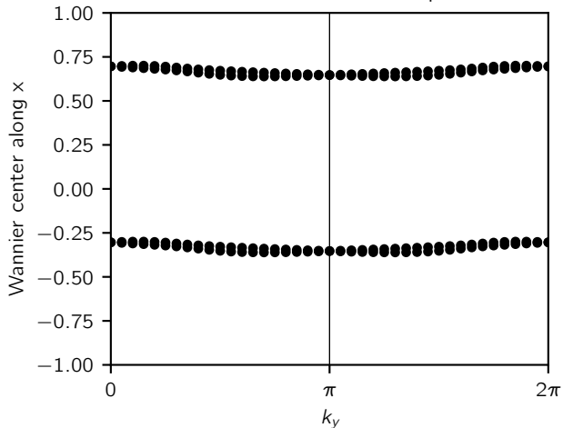
1D Wannier centers: even phase
