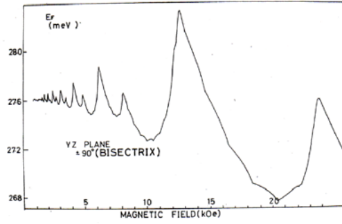
Fig.17 The magnetic field dependence of the Fermi energy ( T = 0 K). Magnetic field is along the Y axis (bisectrix). 9,10
