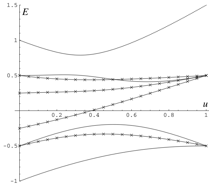
Figure 5. Energies for (P, \sigma, I^{(o)}, S, L) = (0, -1, -1, 0, 1) (cf figures 6 and 7) in units of U - 4T as functions of u = U/(U - 4T) . Levels marked with crosses are twofold degenerate with respect to \sigma = \pm 1 . They also correspond to (P, \sigma, I^{(o)}, S, L) = (0, 1, -1, 0, 1) (equation (5.37)). Upside down the figure shows levels for the same set of quantum numbers with S \leftrightarrow L (equation (5.38)). Note the nondegenerate levels.
