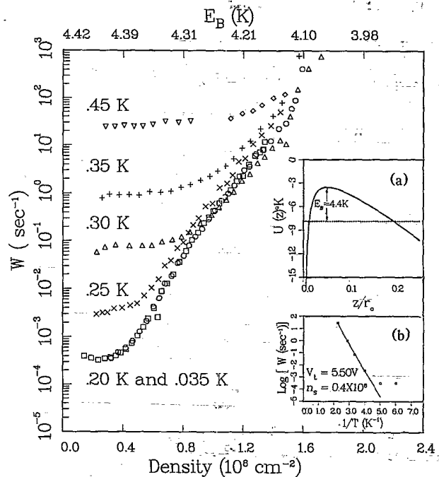
FIG. 2. Temperature dependence of electron escape rates for V_t^b = 5.5 V. Inset (a) illustrates the CHM barrier and metastable state for V_t^b = 5.5 V and n_s = 0.4 \times 10^8 \text{ cm}^{-2} . In inset (b) we plot the measured thermal activation rates ( \square ), together with the two-parameter fit by Eq. (3), solid line.
