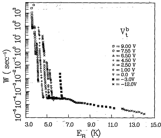
FIG. 3. Escape rates W (data of Fig. 1) as a function of barrier height E_B at T = 40 mK for a series of voltages V_t^b .
