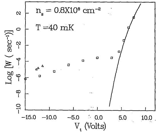
FIG. 4. Escape rates W (data of Fig. 1) as a function of the top plate voltage V_t^b for the electronic density 0.8 \times 10^8 \text{ cm}^{-2} and temperature 40 mK. \square , rates measured in this work; \triangle , rates reported in Ref. [3]; solid line, calculated rates in the correlation-hole model.
