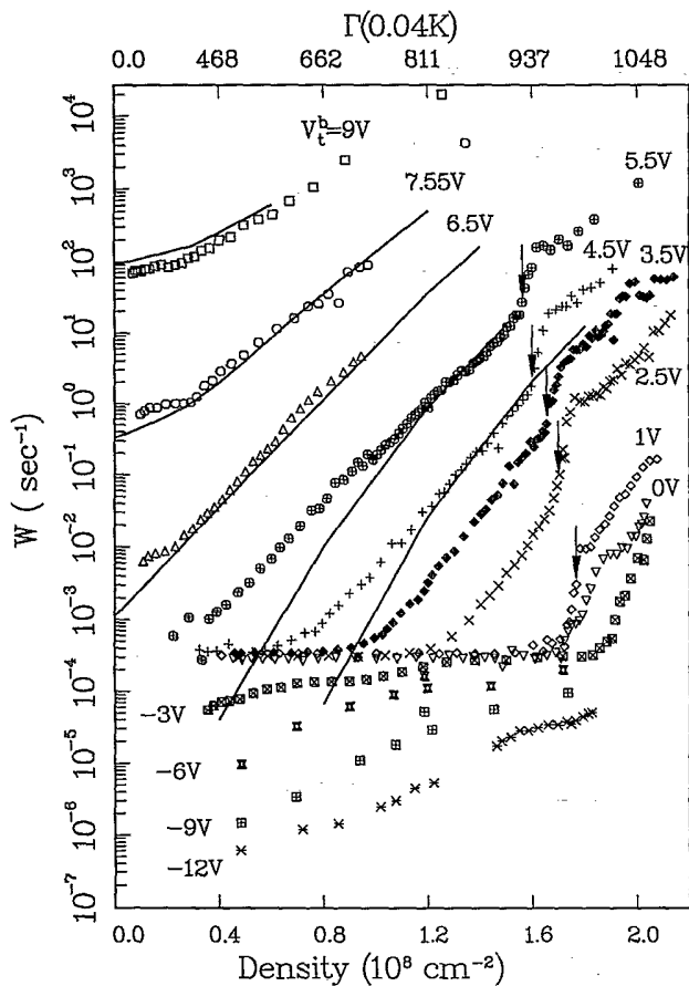
FIG. 1. Density dependence of the escape rates W at T=40 mK for a series of fixed top plate voltages V_t^b . The solid lines are linear interpolations between calculated tunneling rates at discrete values of n_s , for V_t^b = 9, 7.5, 6.5, 5.5, and 4.5 V. Vertical arrows indicate the positions of n_c for V_t^b = 5.5, 4.5, 3.5, 2.5, and 1 V.
