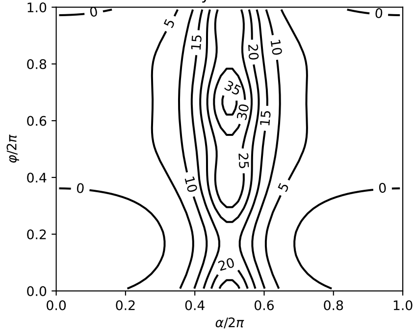
Berry curvature
