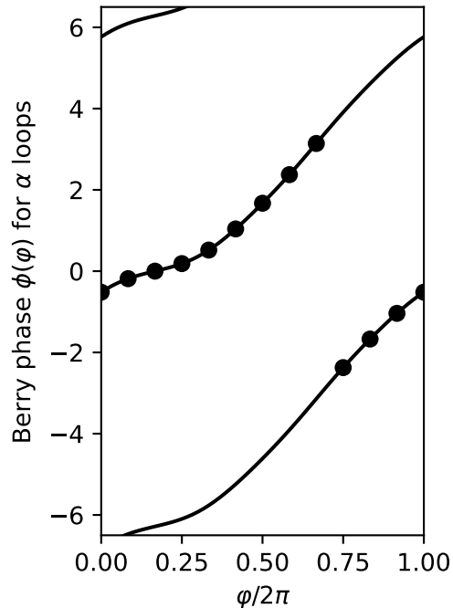
Berry phase
