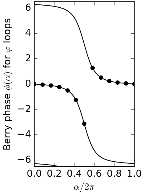
Berry phase
