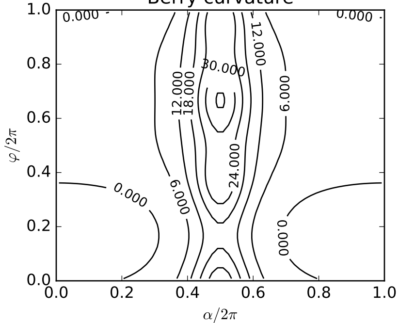
Berry curvature
