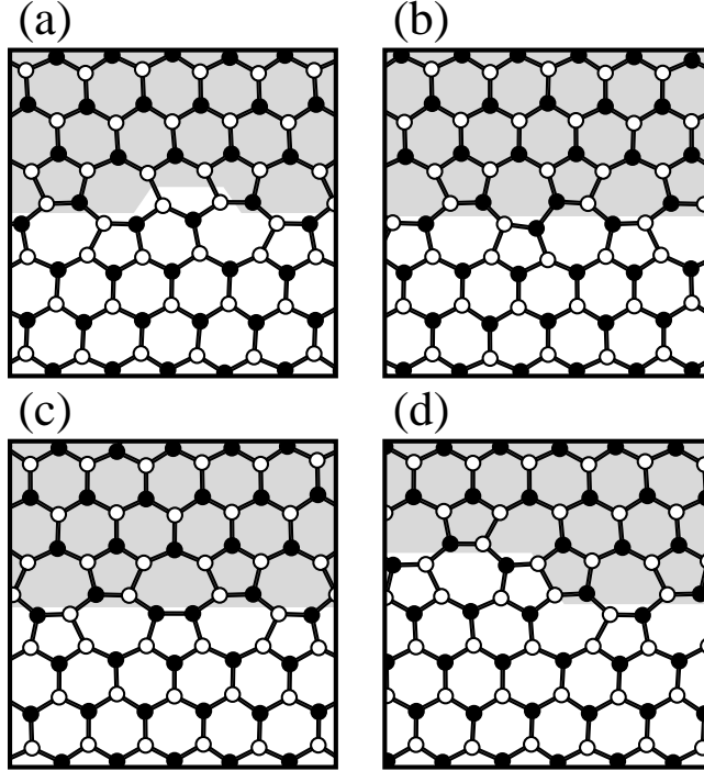
FIG. 3. Examples of several types of core defects in the DP structure. Viewpoint is the same as for figure 1. (a) Phase-switching defect (PSD). (b)-(c) Direction-switching defects (DSD). (d) Kink.
