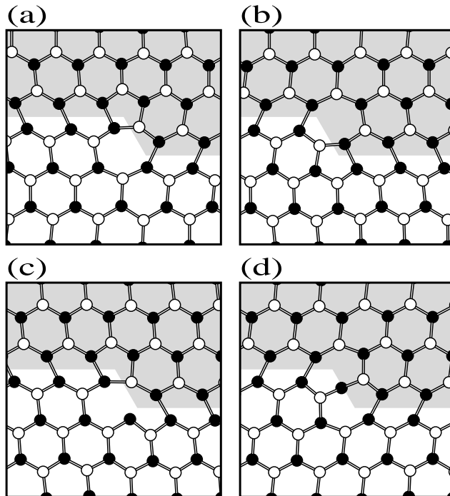
FIG. 2. Core structure of kinks and soliton-kink complexes in the SP core. See text for notation. (a) LR kink. (b) RL kink. (c) LL complex = LR + soliton. (d) RR complex = RL + soliton.
