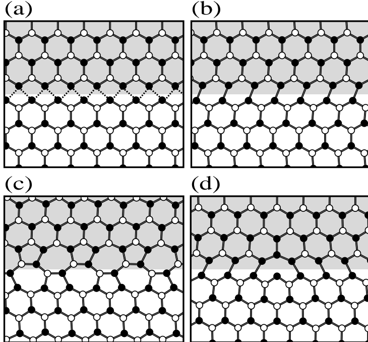
FIG. 1. Models of core reconstruction of the 90^\circ partial dislocation. (a) Symmetric QF reconstruction. (b) Symmetry-breaking SP structure. (c) Ground state symmetry-breaking DP structure. (d) Soliton in the SP core.
