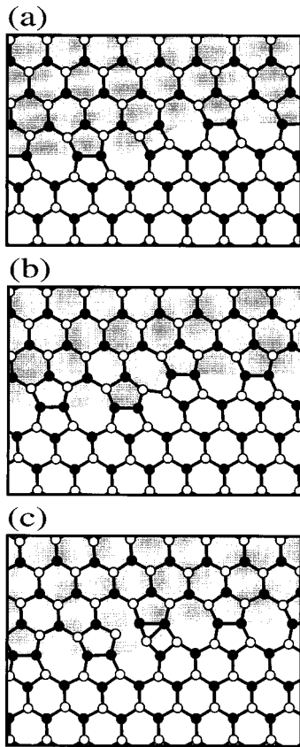
FIG. 3. Core structure of the left kinks in the 30^\circ partial, and associated transition state. Kink notation is explained in the text. (a) LK. (b) LK'. (c) Transition state for the LK \rightarrow LK' transformation.
