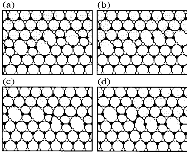
FIG. 6. Core structure of kink-PSD complexes in the 30^\circ partial. In each case, two states of the complex are considered, as explained in the text. (a) LC(0)=LK+PSD at zero separation. (b) LC(1)=LK+PSD one lattice period apart. (c) RC(0)=RK+PSD at zero separation. (d) RC(1)=RK+PSD one lattice period apart.
