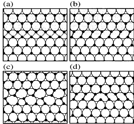
FIG. 7. Models for core reconstruction of the 90^\circ partial dislocation. (a) Symmetric QF reconstruction. (b) Symmetry-breaking SP structure. (c) Ground-state symmetry-breaking DP structure. (d) Reconstruction defect or DSD in the SP core.
