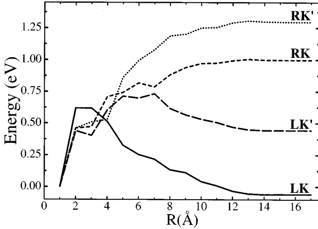
FIG. 5. Keating energy for 30^\circ -partial kinks, using parameters of Qian and Chadi (Ref. 38). Energy E(R) is the sum over all atoms within a distance R from the dislocation core. Corresponding core energy is subtracted to yield defect energies.
