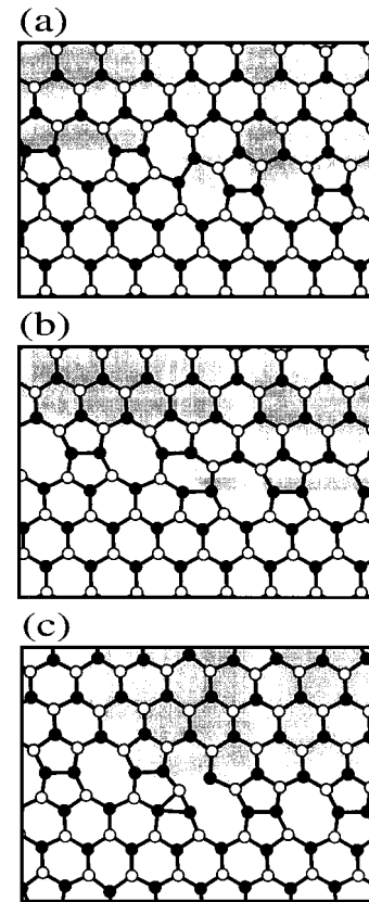
FIG. 4. Core structure and transition state of right kinks in the 30^\circ partial. Kink notation is explained in the text. (a) RK. (b) RK'. (c) Transition state for the RK \rightarrow RK' transformation.
