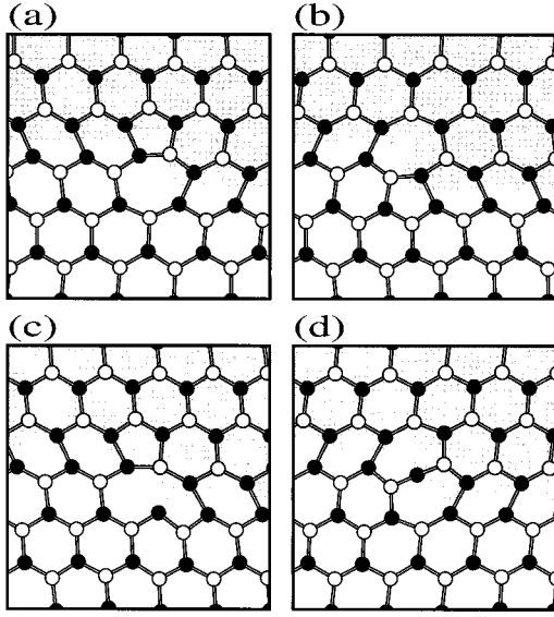
FIG. 8. Core structure of kinks and DSD-kink complexes in the SP core. See text for notation. (a) LR. (b) RL. (c) LL complex = LR + DSD. (d) RR complex = LR(RL) + DSD.
