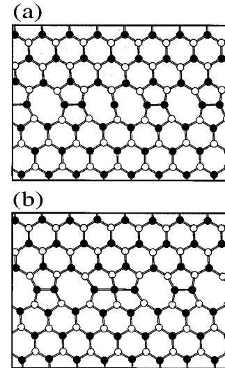
FIG. 2. (a) Core structure of a phase-switching defect (PSD), which is a reconstruction defect in the core 30^\circ -partial dislocation. The phase of the reconstructed bond along the dislocation line is switched, going through the defect. (b) Saddle-point configuration for the propagation of a PSD along the core.
