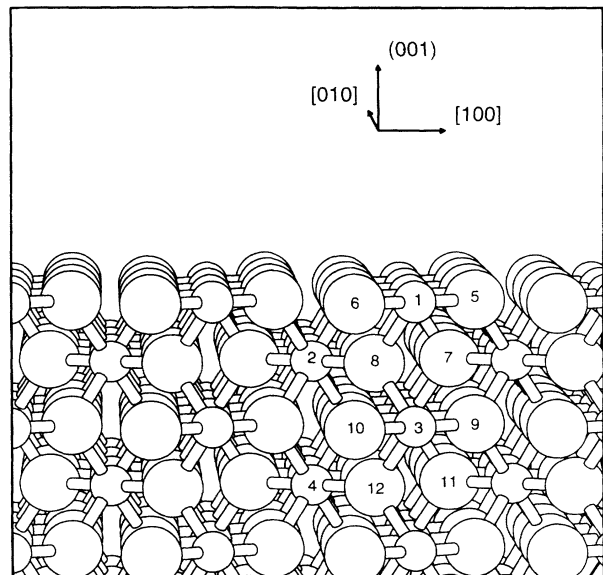
FIG. 5. The structure of the unrelaxed stoichiometric (001) surface.
