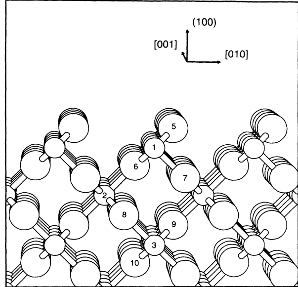
FIG. 3. The structure of the unrelaxed stoichiometric (100) surface.
