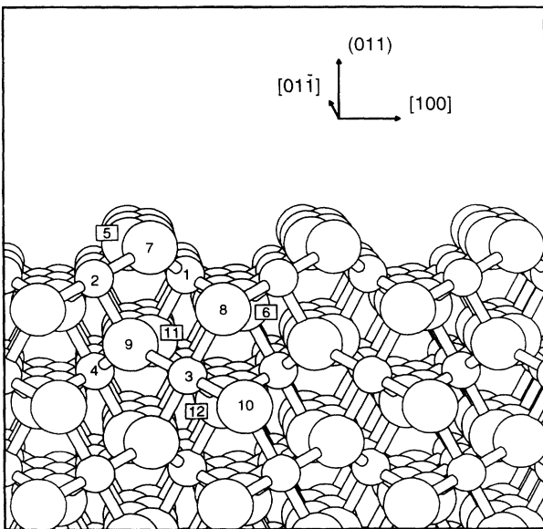
FIG. 4. The structure of the unrelaxed stoichiometric (011) surface.
