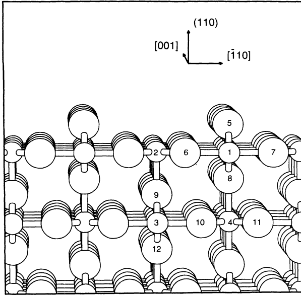
FIG. 2. The structure of the unrelaxed stoichiometric (110) surface.
