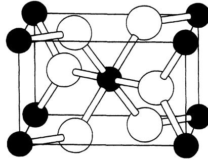
FIG. 1. The structure of bulk \text{TiO}_2 .
