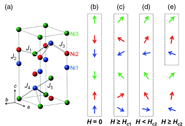
FIG. 1 (color online). (a) Crystal structure of \text{Ni}_3\text{TeO}_6 . Only Ni ions are shown. (b)–(e) Schematic spin structure along a c -axis chain at different magnetic fields applied along the c axis. The spins in the buckled honeycomb planes are aligned ferromagnetically in zero magnetic field [13]. J_i stands for the five nearest-neighbor exchange constants considered in the text. Dotted boxes indicate the magnetic unit cell along the c axis, which is doubled for (b)–(d) but not for (e).
