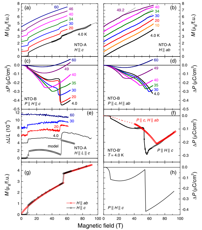
FIG. 2 (color online). (a),(b) Magnetization and (c),(d) change of electric polarization ( \Delta P ) of \text{Ni}_3\text{TeO}_6 for magnetic fields applied along different crystalline axes as indicated. (e) c -axis magnetostriction as a function of magnetic field applied along the c axis. Solid lines are experimental data taken under isothermal condition and open squares are from model calculations based on parameters shown in Table I. (f) \Delta P measured up to 92 T for H\parallel ab and H\parallel c . (g), (h) The magnetic field dependence of M and \Delta P along the c -axis in H\parallel c configuration obtained from the model calculations described in text. Dashed lines in (a) and (b) are guides for the eyes. (a),(b) magnetization and (e) magnetostriction curves are shifted for clarity. (e) Jump in magnetostriction at H_{c2} shows a slight difference in magnitude between the different types of magnets used, possibly due to the variation in magnetic field sweep rate. (f) Lines and open symbols denote data taken by using a capacitor-bank-driven and a hybrid pulse magnet, respectively. A single domain sample was used for (c) and (d) while a multidomain (as-grown) sample was used for (f).
