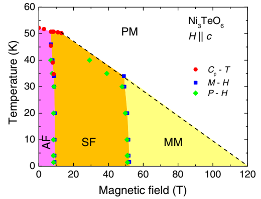
FIG. 3 (color online). H - T phase diagram of \text{Ni}_3\text{TeO}_6 with magnetic field applied along the c axis determined by peak positions in dM/dH , \alpha \equiv dP/dH , and specific heat (see Supplemental Material [18]) data. Dashed line is a guide for the eyes.
